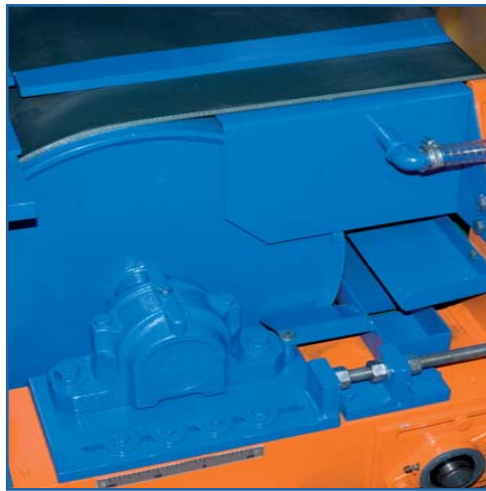
Tiles containment guides, belt belt tightening saddle and belt washing. Guías sujeción balbosa durante el recorrido, banda, tensor y tubo lavado banda.
