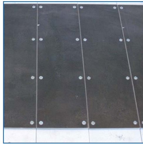
Plates for layng, belt realized in special metal anti wear and easily interchangeable. Placa plano soporte banda en acero especial antidesgaste, fácilmente intercambiables.
